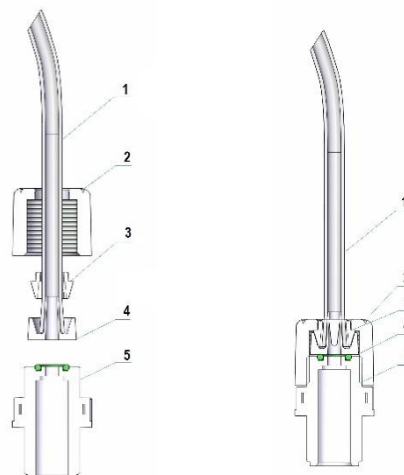
Fig.4 – Raccordement hydraulique
