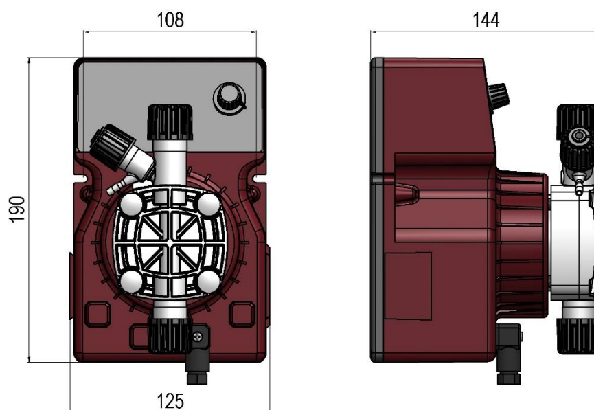
Fig. 1a – PMF pump, wall fixing (dimensions indicated in mm.).
